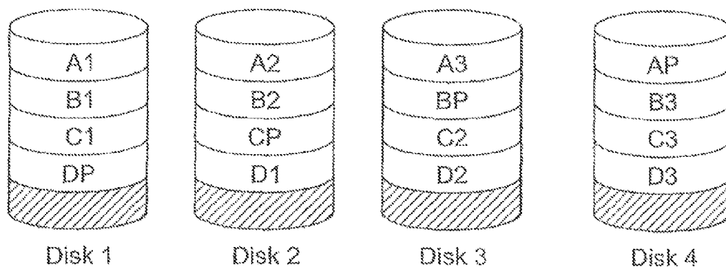
FIG. 1C (Prior Art)
